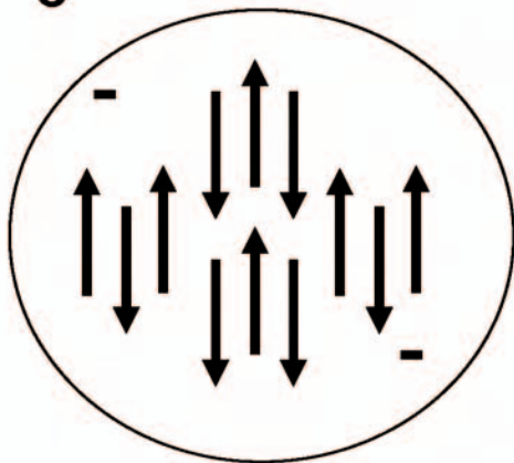
He atom
