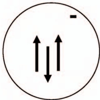
H atom
